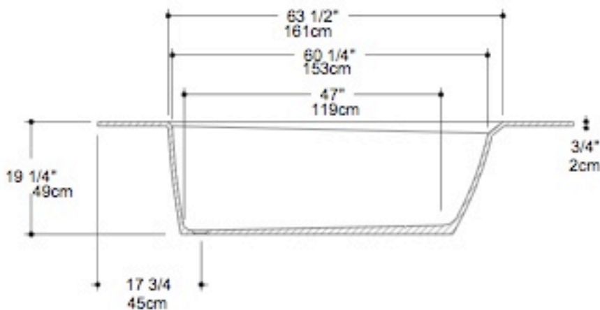
SQUARE DECK AS DEMOLDED FROM AN UNLOCKED MOLD
